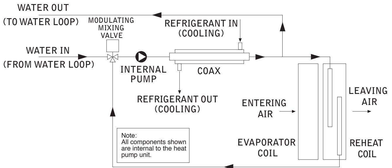
Figure 1: ClimaDry® Schematic
